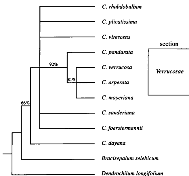
Fig. 3. Bootstrap consensus of 2 trees from parsimony analysis of ITS1-5.8S-ITS2 sequences (only percentages >50% are given).
