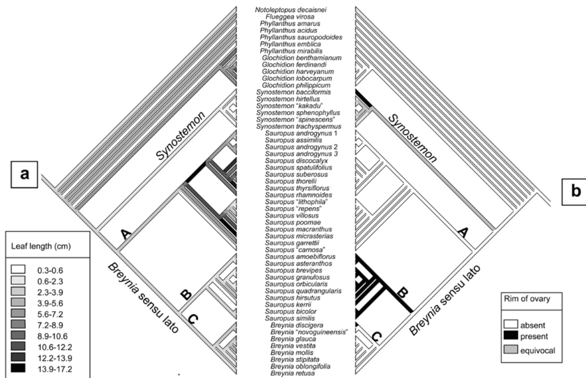
Fig. 4.3. Character state transformations in a. leaf size and b. presence of a rim at the edge of the ovary. Clade A and B are species of Sauropus and Clade C species of Breynea .
